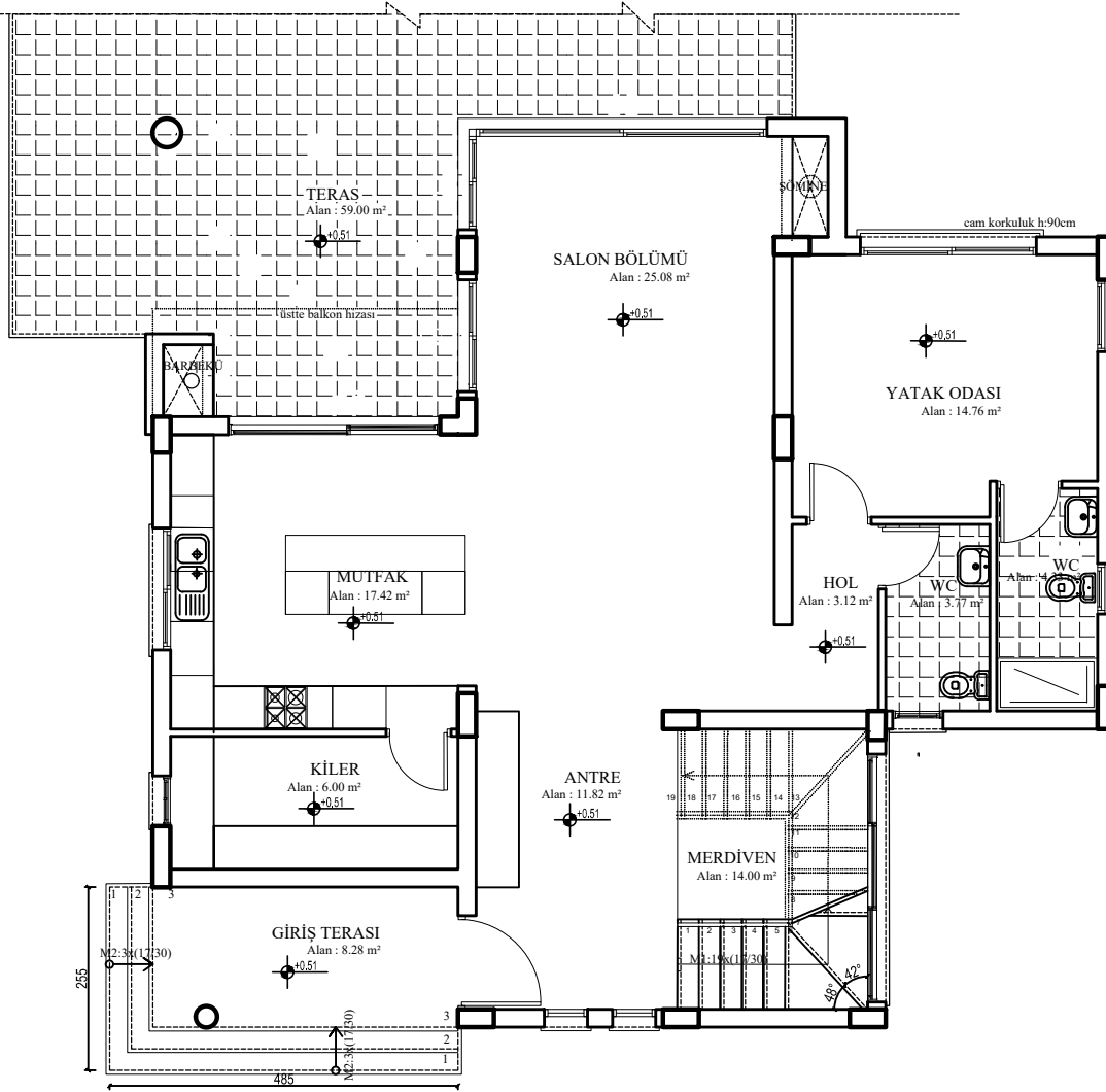
C BLOK (C1-C2-C3-C4-C5) ZEMİN KAT PLANI ÖLÇEK:1/50
