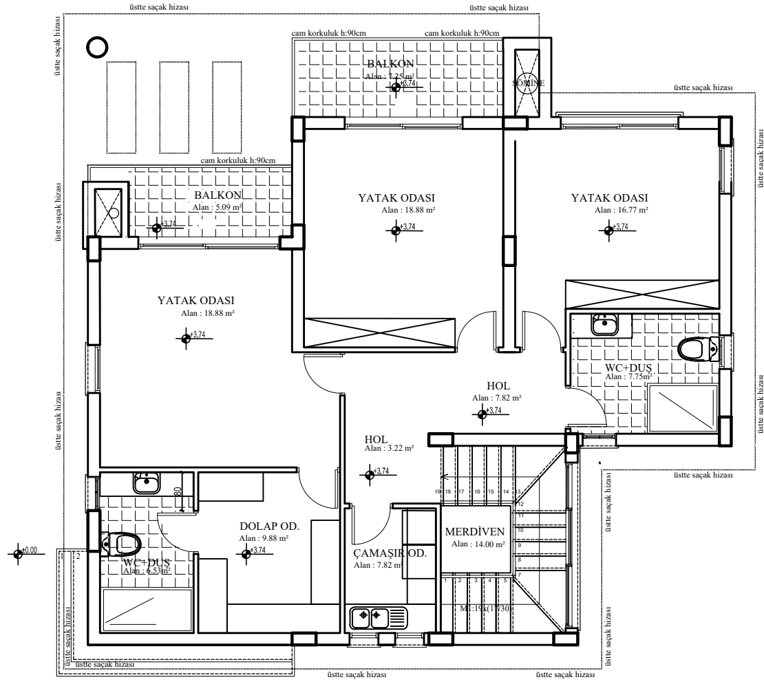
C BLOK (C1-C2-C3-C4-C5) BİRİNCİ KAT PLANI ÖLÇEK:1/50
